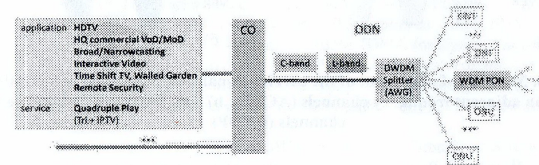
Pic. 7. Option of hybrid N-OFDM-X-PON
