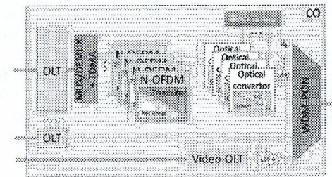
Pic. 6. Structure of CO using N-OFDM
