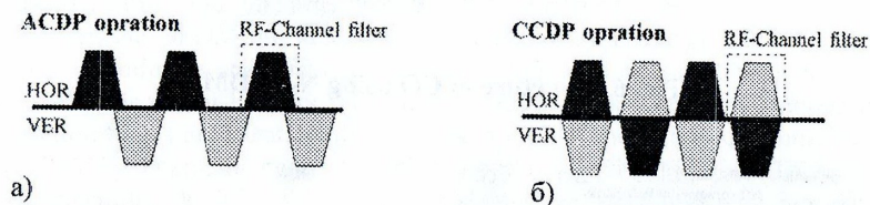
Pic. 8. Methods of alignment of the carrier signal frequency dual polarization: a) – on adjacent frequency channels (ACDP); b) – on the combined frequency channels (CCDP)
