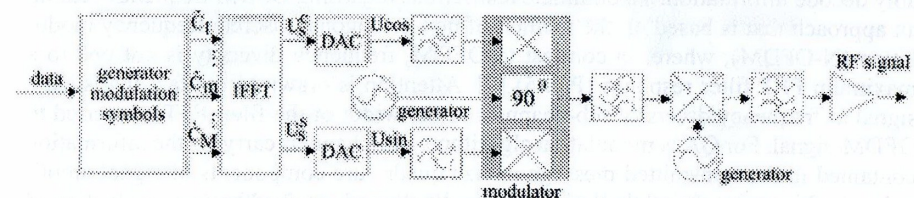
Fig. 3. Scheme of formation OFDM (SOOFDM) for transferring party
