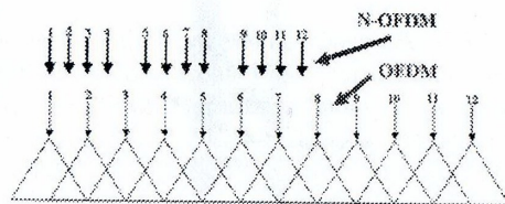
Pic. 5. The arrangement of N-OFDM (OFDM) signal
